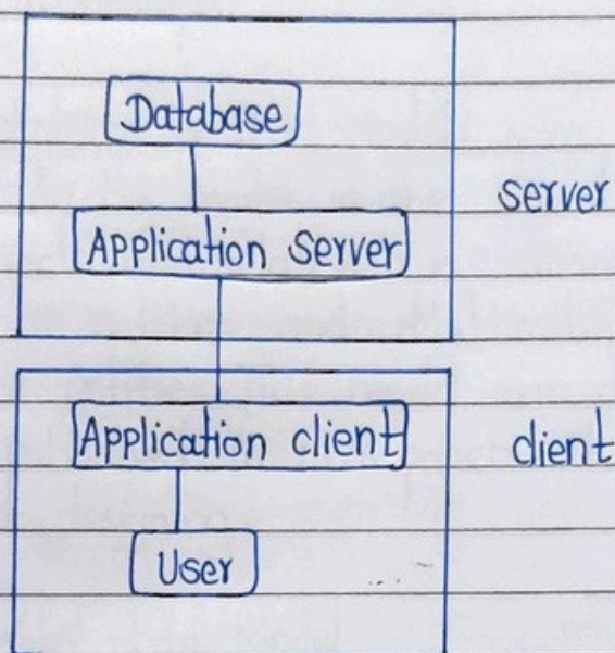
Fig 3-tier Architecture
