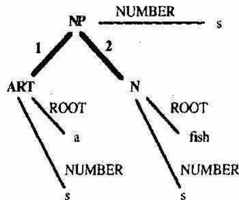
Figure 4.1 Viewing a feature structure as an extended parse tree
